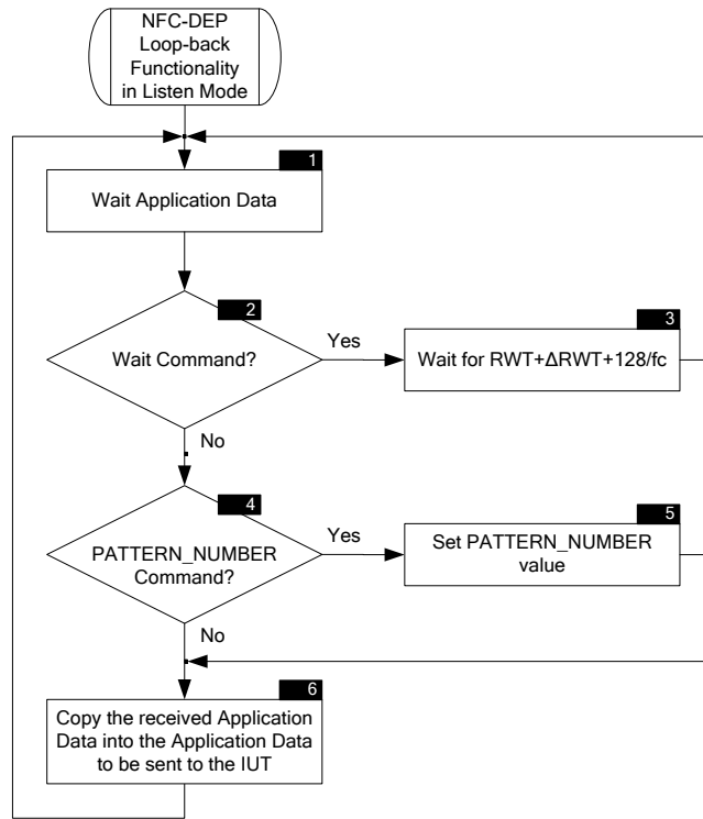
Figure 20: NFC-DEP Loop-back Functionality in Listen Mode Flowchart
