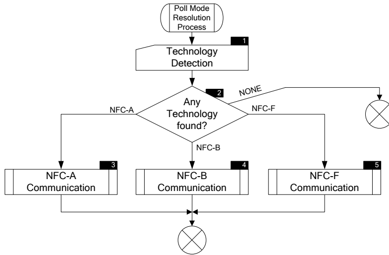
Figure 4: Test Profile – Poll Mode Resolution Process Flowchart – Main Flow
