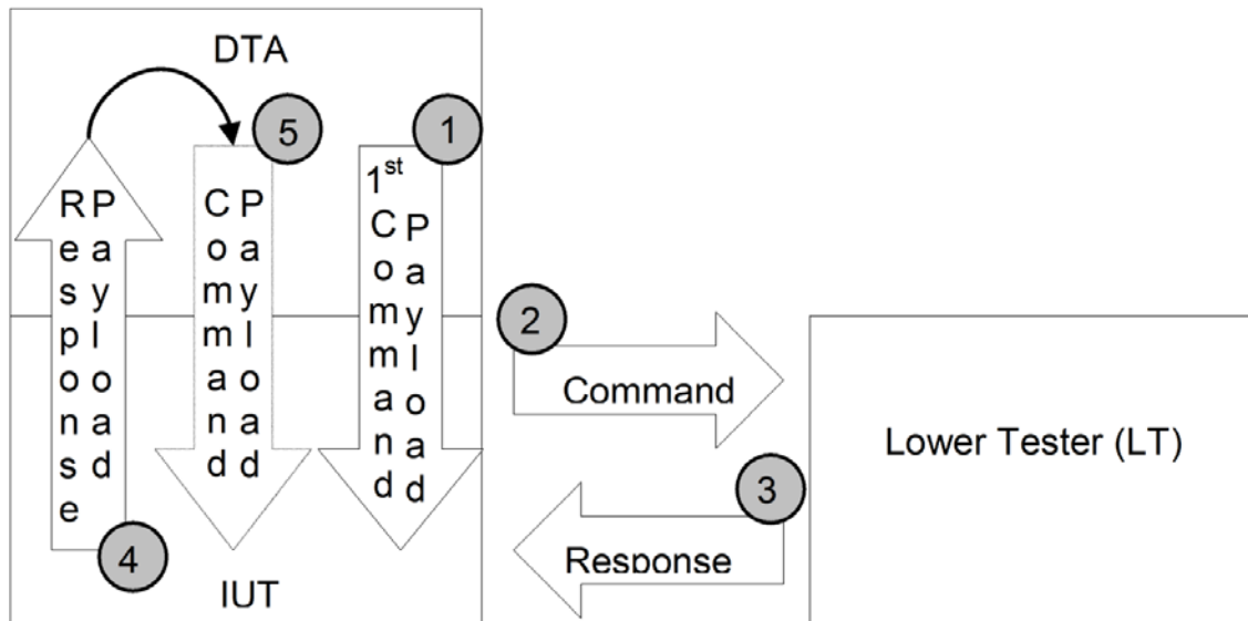
Figure 13: Loop-back Test Functionality in Poll Mode
