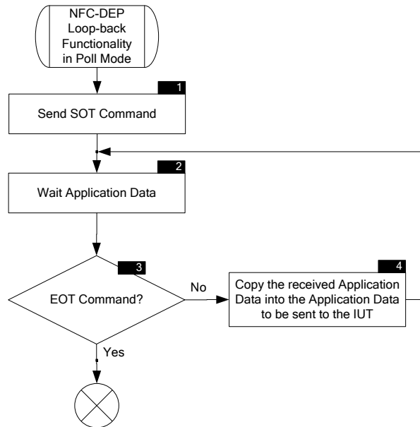
Figure 16: NFC-DEP Loop-back Functionality in Poll Mode Flowchart
