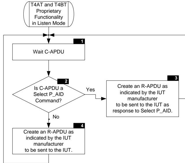
Figure 22: T4AT and T4BT Proprietary Functionality in Listen Mode Flowchart
